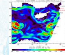
Figure 11: Surface model current Vs buoys trajectories (up), distance error results (down)
