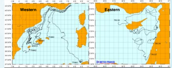
Figure 3 : Drift experiments used as reference cases, for Western (left) and Eastern (right) Mediterranean.
